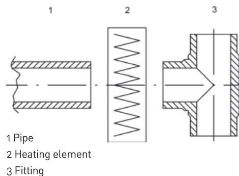
The principle of fusion jointing
