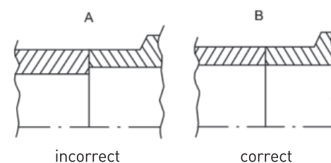
Join only components with similar wall thicknesses
