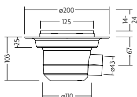
Quad Gravity Drain Tiled Insert 14mm - Horizontal Outlet
