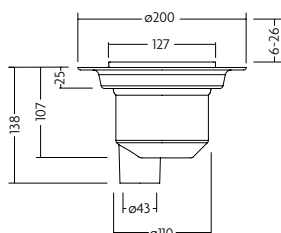
Quad Gravity Drain Slot - Vertical Outlet
