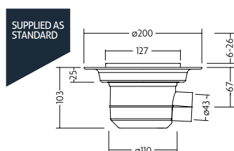
Quad Gravity Drain Slot - Horizontal Outlet
