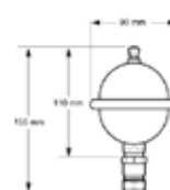
Surge Damper
