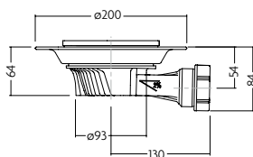
Tiled Drain Slim+ Horizontal Slot
